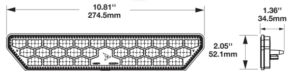
Post Mounted
