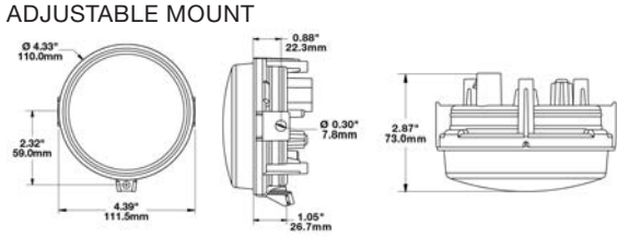
ADJUSTABLE MOUNT
