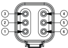
View: Back of Lamp 6-Pin Deutsch
