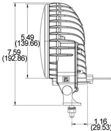
Dimensions in inches (mm in parentheses). Dimensions are for reference only.
