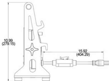
Dimensions in inches (mm in parentheses). Dimensions are for reference only.
