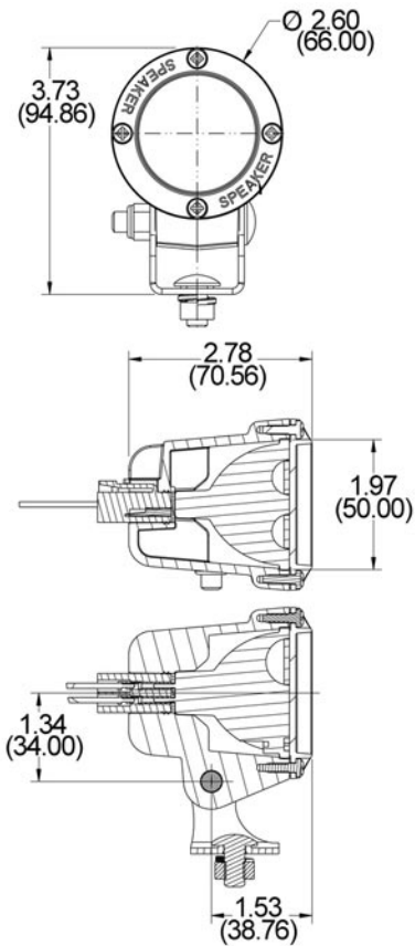
Dimensions in inches (mm in parentheses). Dimensions are for reference only.
