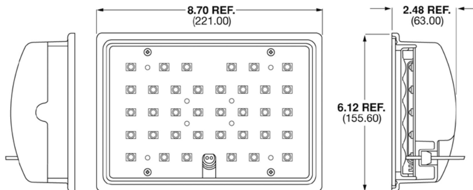
Model 524 Dimensions
